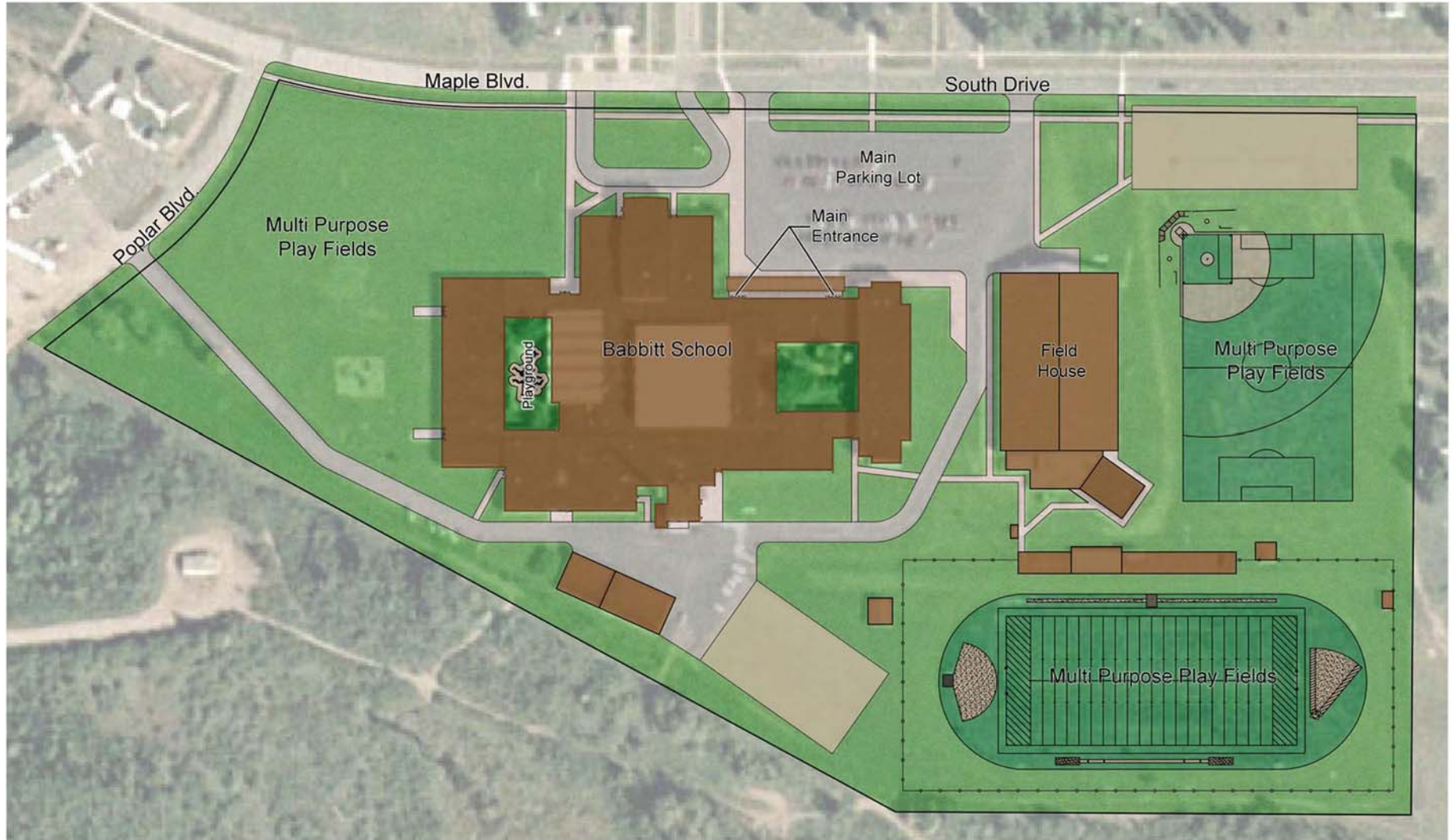
Proposed Site Plan ISD 2142 Babbitt-Embarrass Tower-Soudan One-Section PK-12 School
